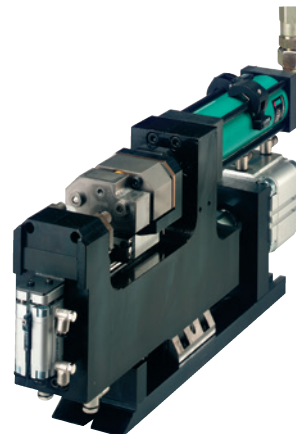
Punching tongs with TOX®-Hydraulic Cylinder
