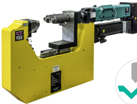
Machine tongs with TOX®-ElectricDrive
